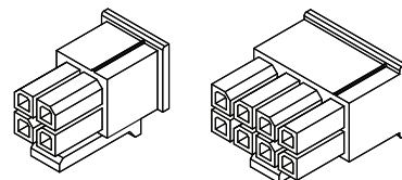
4-pin and 8-pin connectors are supplied on the end of 8" leads.
