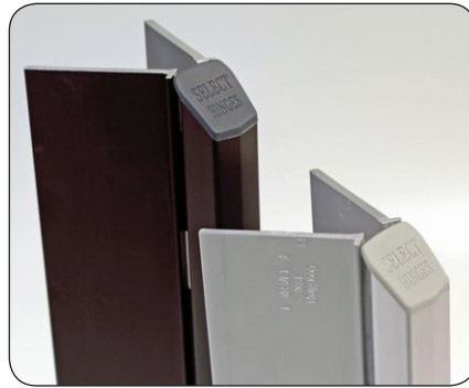
SELECT's ligature-resistant hospital tip [HT] on concealed geared continuous hinges.
