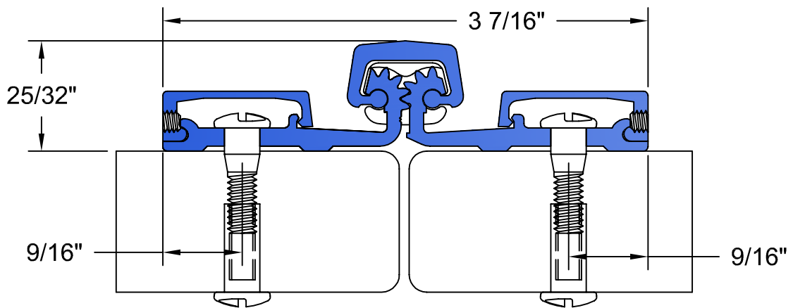
SL60/SL62 DOOR AND FRAME MOUNT FLUSH
